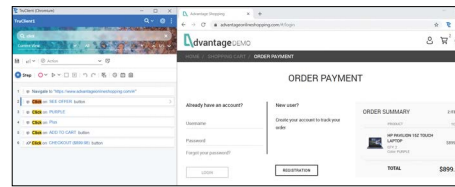
Figure 2. The patented Micro Focus TruClient technology provides a browser-embedded, interactive way of scripting next-generation Web-based applications
